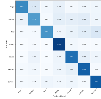
Fig. 2: Confusion Matrix for RAF-DB
